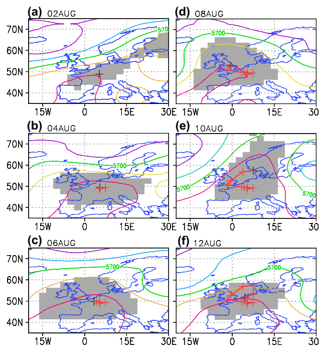
Fig. 6 Same as Fig. 3, but for persistent strong open ridges that occurred 2–12 August 2003 and caused the record heatwave in Western Europe
