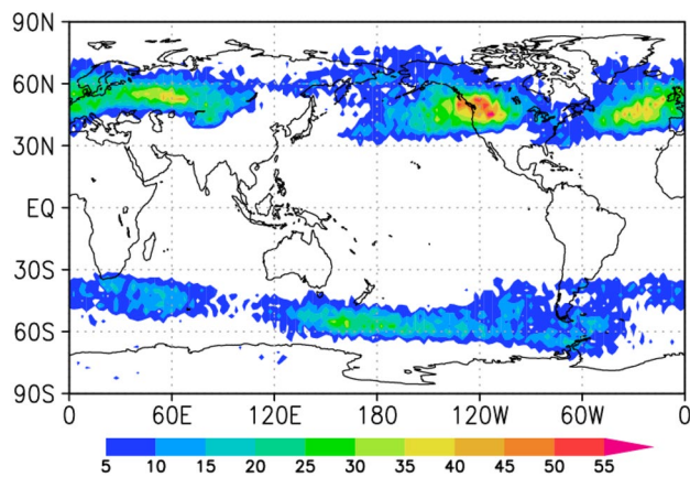
Fig. 11 Total number of PMZ cores during 1979–2015
